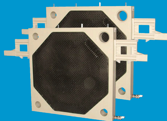
Squeeze Membrane
